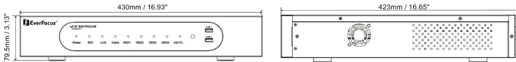
Front view
