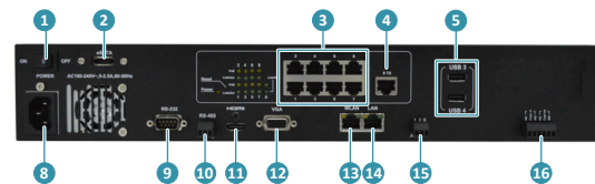
Rear view
